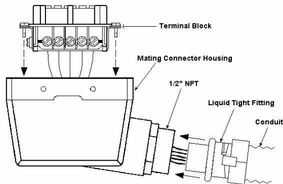
Figure 8: Sealed Industrial Latching Connector
